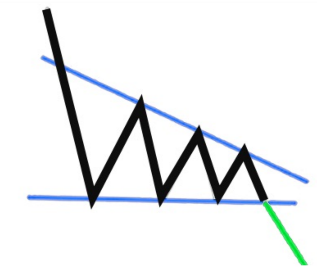
Ascending Triangle
